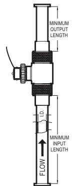
Vertical Mount
